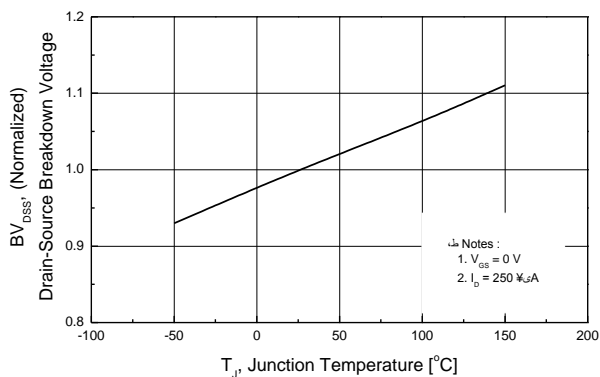
Fig 7. Breakdown Voltage Variation vs. Junction Temperature
